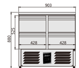
GTS-S901 S/SGTS- Top 4×GN1/2
